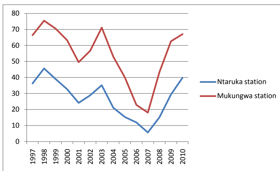
Figure 2. Power production from the Ntaruka and Mukungwa hydropower stations (GWh/Annum) (RECO, 2011)
